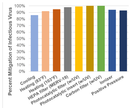
Figure 22C: Total Mitigation of Viral Output on Buses
