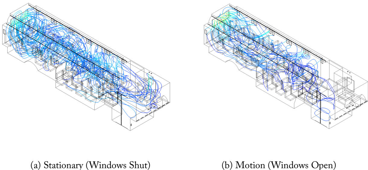
Figure 13. Comparison of Numerical Airflow and Circulation Patterns Inside the Stationary (Windows Shut) and Moving (Windows Open) Bus A
